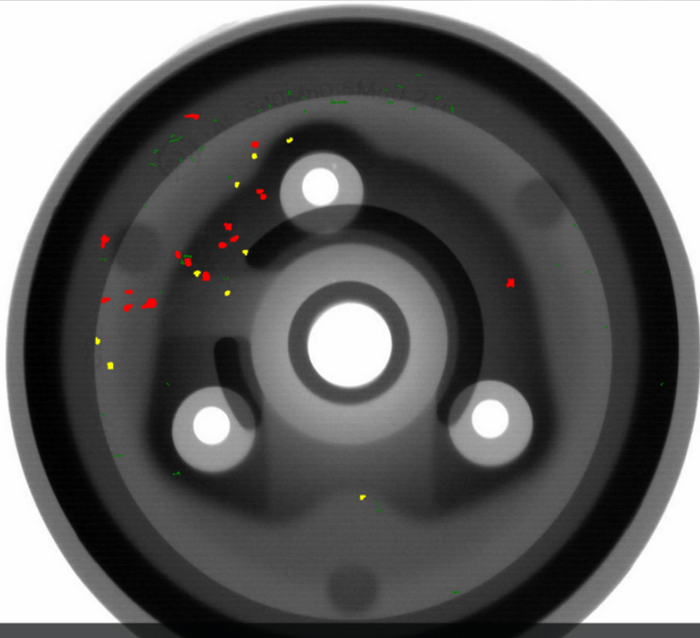
DEFECT IDENTIFICATION & CLASSIFICATION IN DIFFUSER PLATE
