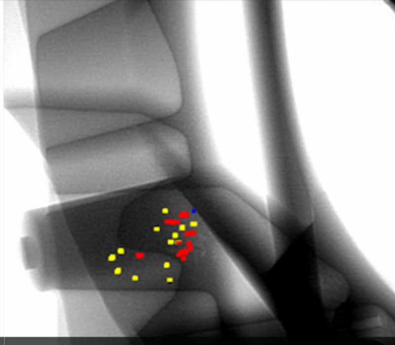
DEFECT IDENTIFICATION & CLASSIFICATION IN SWING ARM
